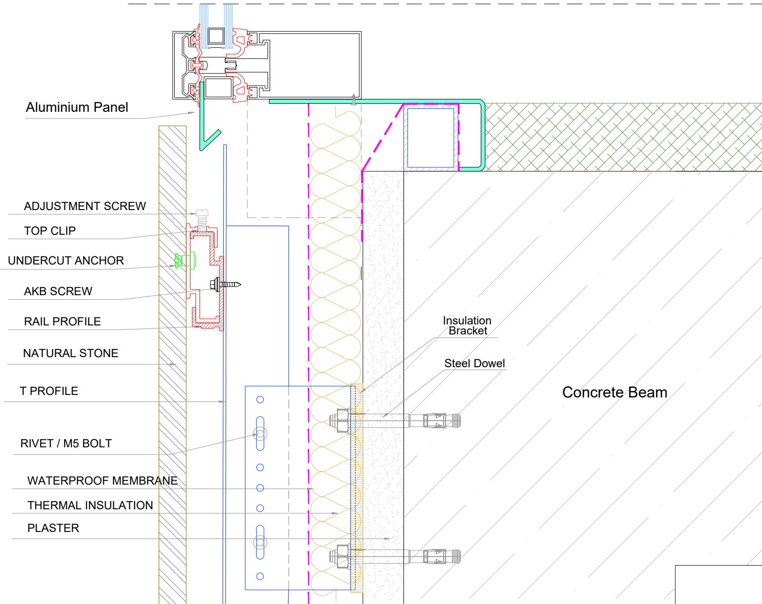
DETAIL C
