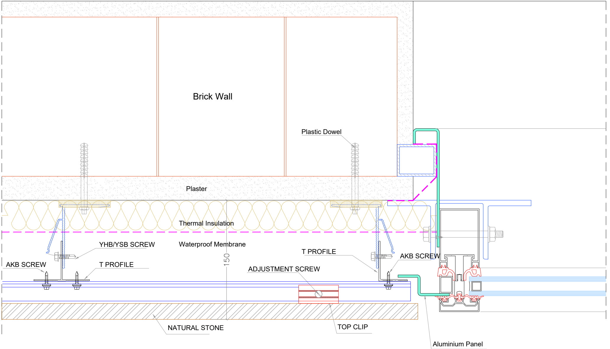
DETAIL A
