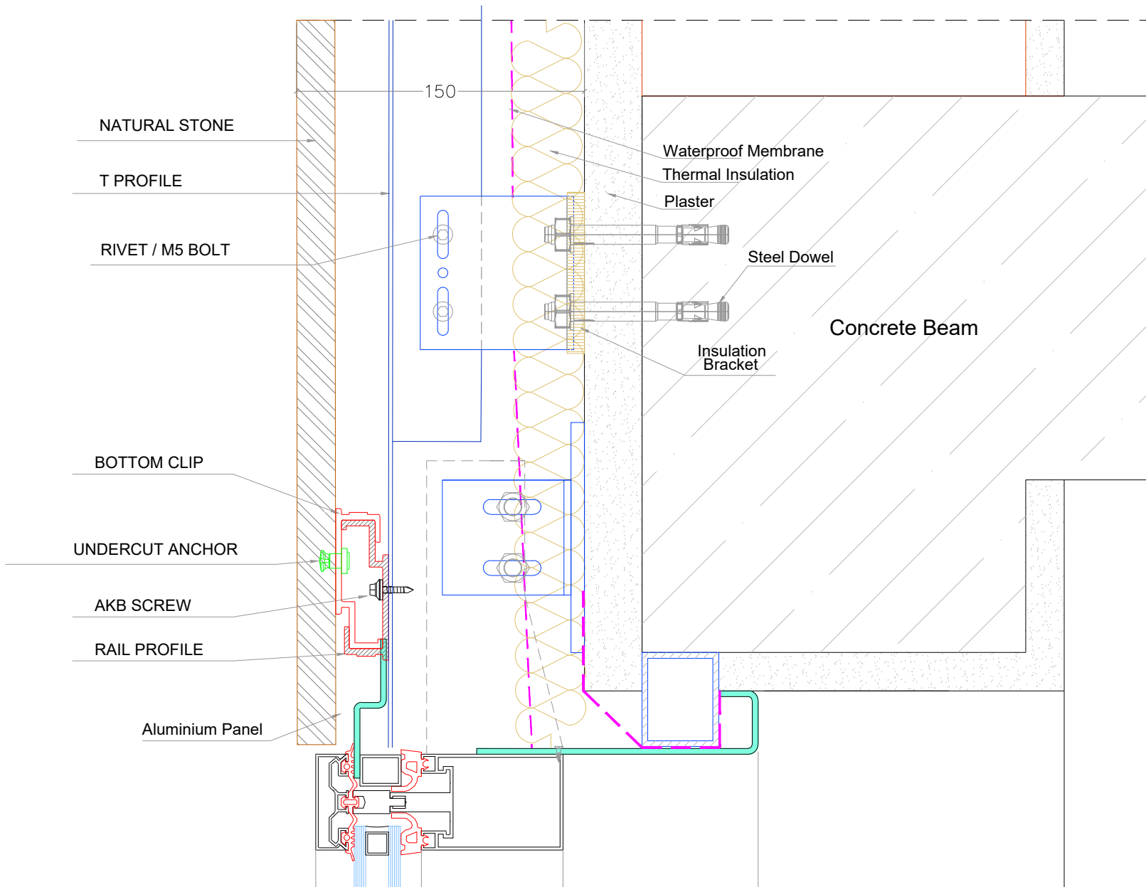
DETAIL B
