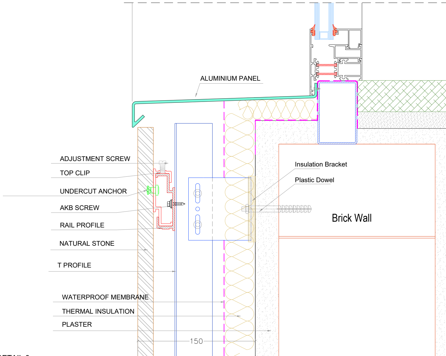
DETAIL 9
