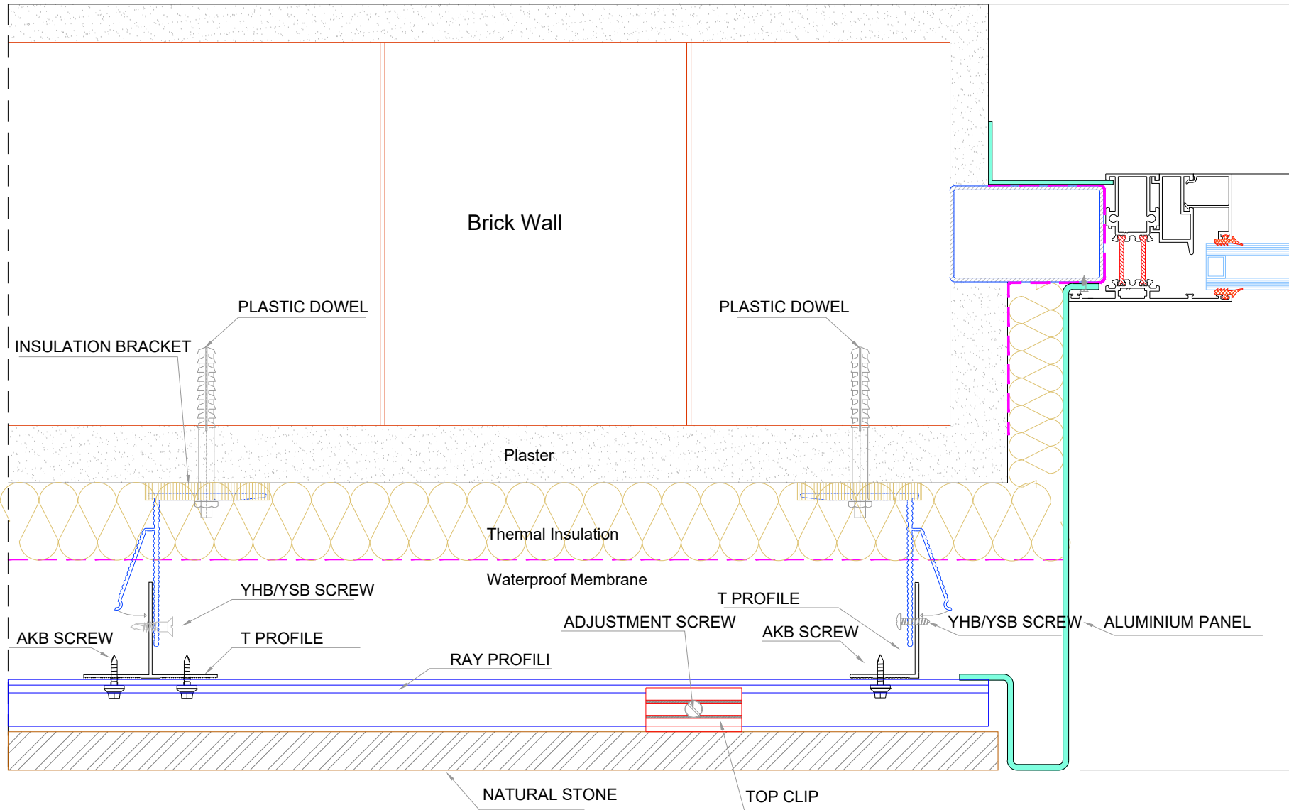
DETAIL 7
